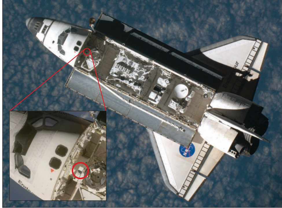
A proximity sensor named DragonEye, developed by SpaceX, underwent flight system trials on the Space Shuttle Endeavour during the STS-127 mission in July 2009. This Laser Imaging Detection and Ranging (LIDAR) sensor system provides three-dimensional images based on the amount of time it takes for a single laser pulse from the sensor to reach a target and bounce back. The successful demonstration provided range and bearing information needed to guide the Dragon spacecraft during future ISS resupply deliveries.
