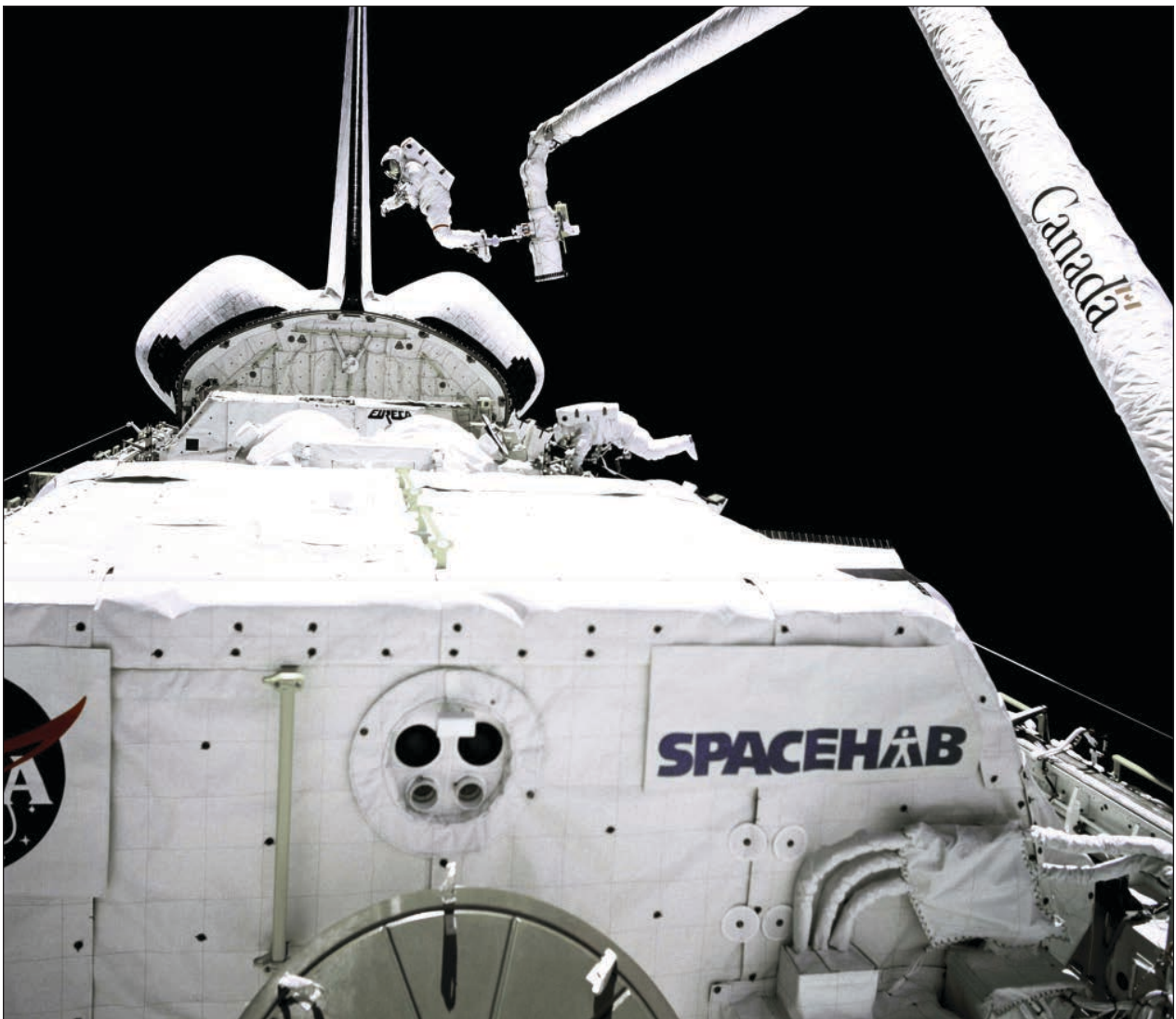
SPACEHAB's first module in space provided a laboratory that more than doubled the pressurized workspace for crew experiments. The inaugural flight of this commercially-developed unit was in June 1993 on the Space Shuttle Endeavour as part of the STS-57 mission.
